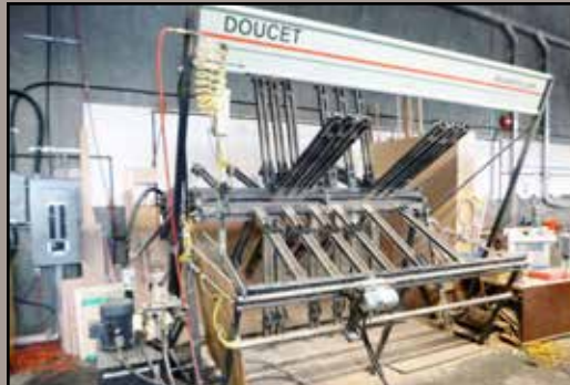
DOUCET SRX-6-8.5-40-R Clamp Carrier
